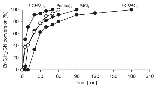
Figure 2. Sonogashira coupling of 1 with 2 catalyzed by homogeneous \text{Pd}(\text{dba})_2 or by the Pd clusters prepared from various precursors. Reaction conditions: 1.5 mmol phenylacetylene, 1.5 mmol TBAA, 1 mol % catalyst (total Pd clusters relative to \text{Br-C}_6\text{H}_4\text{-CN} ), 8 mL DMF, 50 °C, \text{N}_2 atmosphere.
