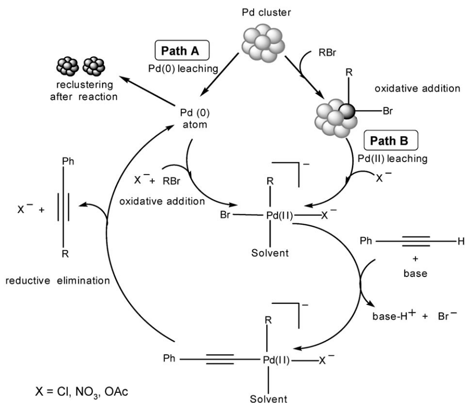
Figure 4. Proposed mechanism for the Pd cluster-catalyzed Sonogashira cross-coupling involving two possible pathways.
