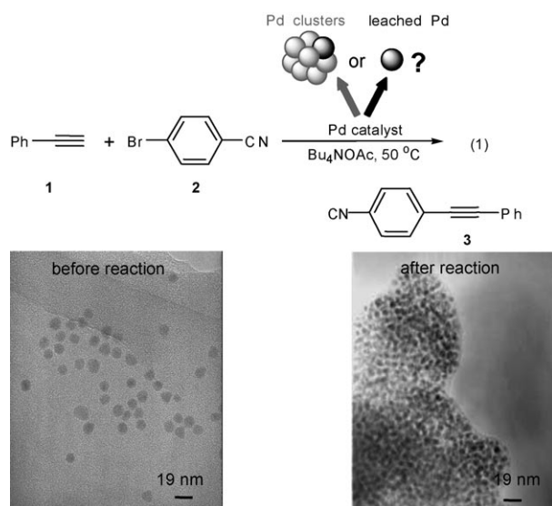
Figure 1. Sonogashira coupling of phenylacetylene with 4-bromobenzonitrile using Pd clusters as catalyst and TEM images before (left) and after (right) the reaction.
