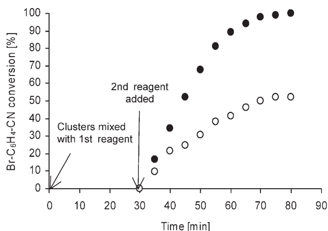
Figure 3. Time-resolved profiles showing the effect of mixing either 4-bromobenzonitrile 1 or phenylacetylene 2 with the Pd clusters prior to reaction. The ‘●’ and ‘○’ symbols denote [ 1 + Pd] with 2 added after 30 min and vice versa , respectively.
